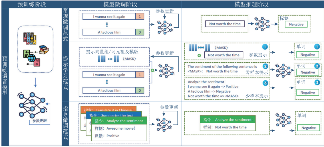
Fig. 2 Three paradigms for deploying LLMs in NLP tasks
