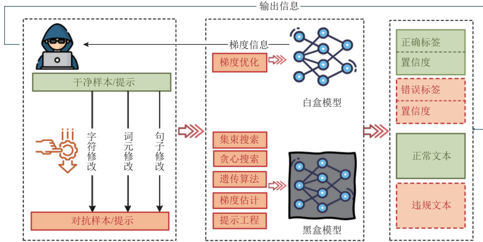
Fig. 4 Illustration of a typical adversarial sample attack
